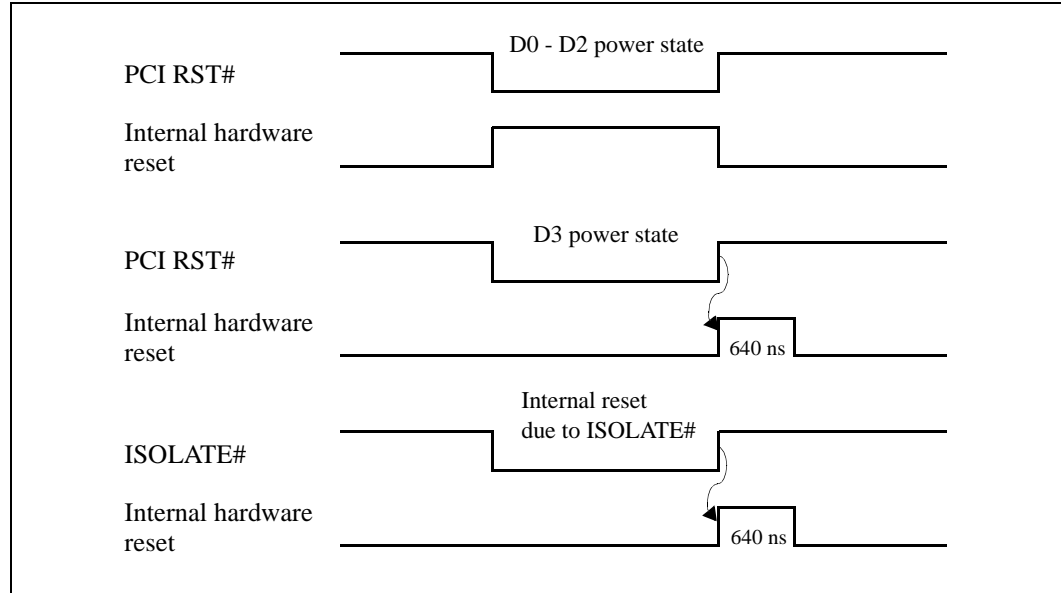
Figure 10. 82559ER Initialization upon PCI RST# and ISOLATE#
